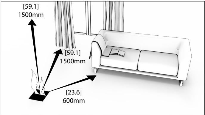
2. Indoor Clearances
